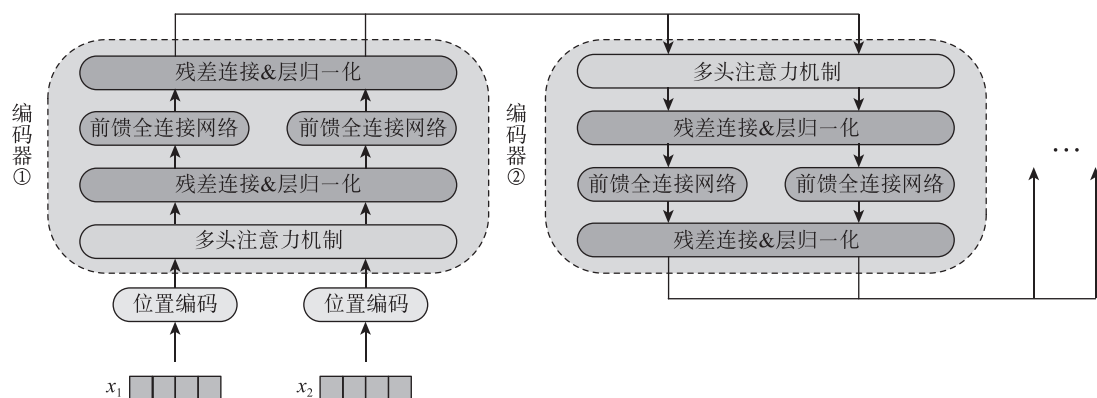
图2 Bert 基本框架 (Transformer Encoder - only)
